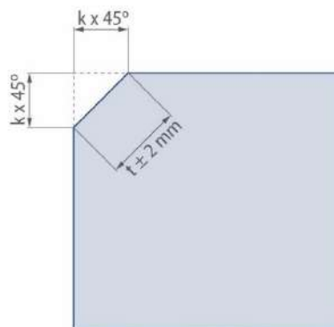
Fig. 17 Corner cut-off
